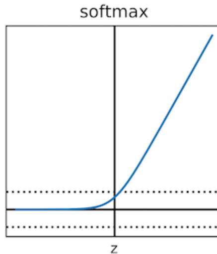
Figure 9: Softmax Function
