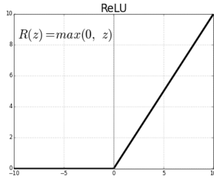
Figure 8: ReLU Function
